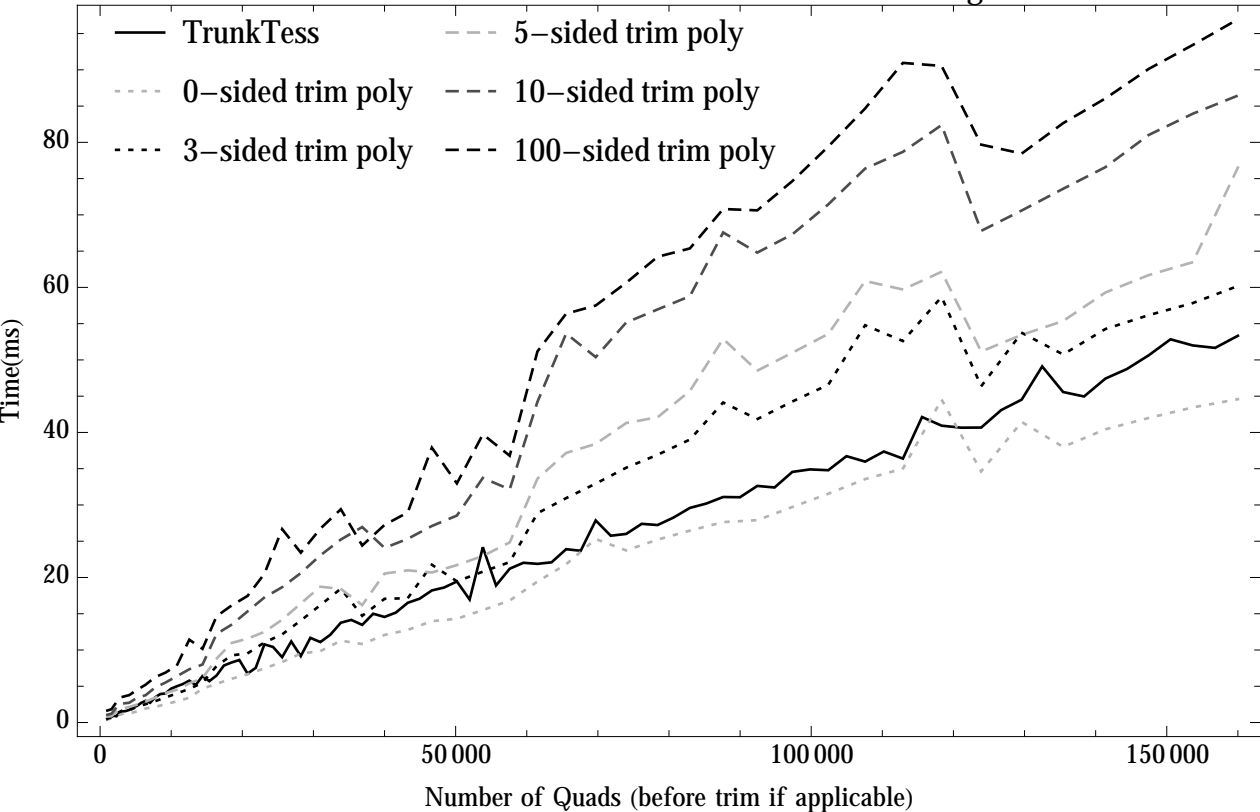
Blender Trunk vs GridMesh Tessellation Timing
